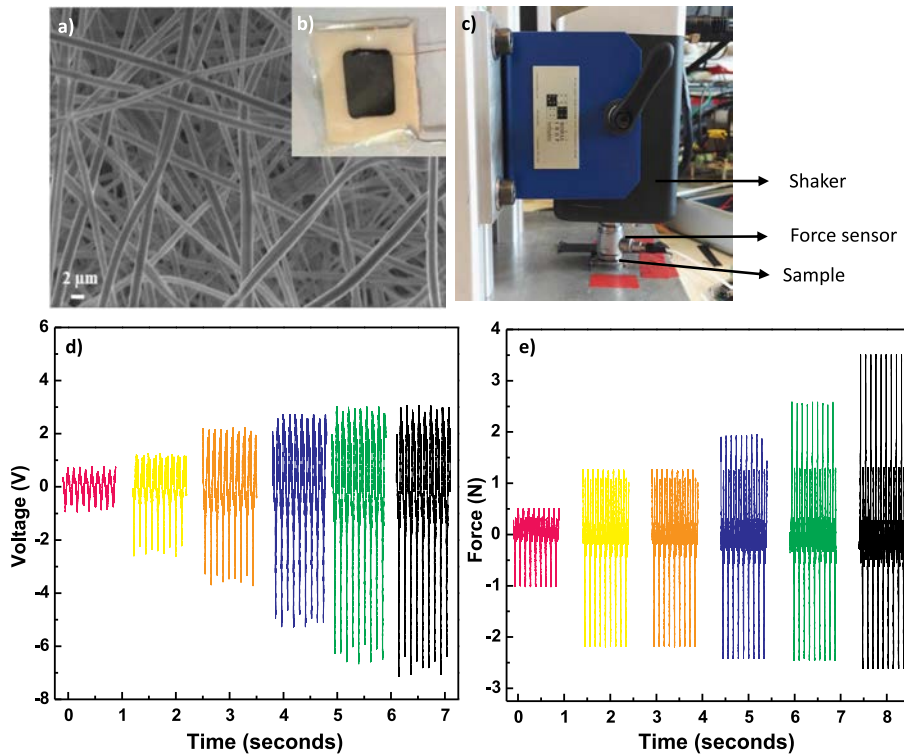
Fig. 8. Performance of the NG under different impact forces (with f = 9 Hz). (a) SEM image of PVDF-TrFE nanofibers showing their surface and structural morphology. (b) Optical image of PVDF-TrFE nanofiber based NG device. (c) Schematic of the used experimental setup. (d, e) The voltage output and applied force of the NG under impact exerted by a shaker.
