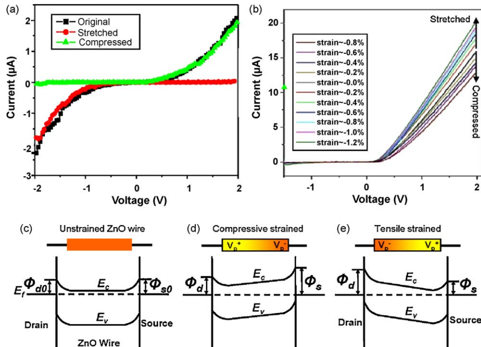
Fig. 9. Piezotronic effect. (a) Changes of the I - V characteristic of a ZnO NW from symmetric (black) to asymmetric rectifying behavior when it's stretched (red) or compressed (green). (b) Change of I - V characteristic of a ZnO NW with rectifying behavior when it's stretched or compressed. Schematic energy band diagram of the unstrained (c), compressive strained (d), and tensile strained (e) NW, showing the different effect of the piezopotential on the Schottky barrier height at drain electrode side and at source electrode side (from Ref. [31,32,35]). (For interpretation of the references to colour in this figure legend, the reader is referred to the web version of the article.)
